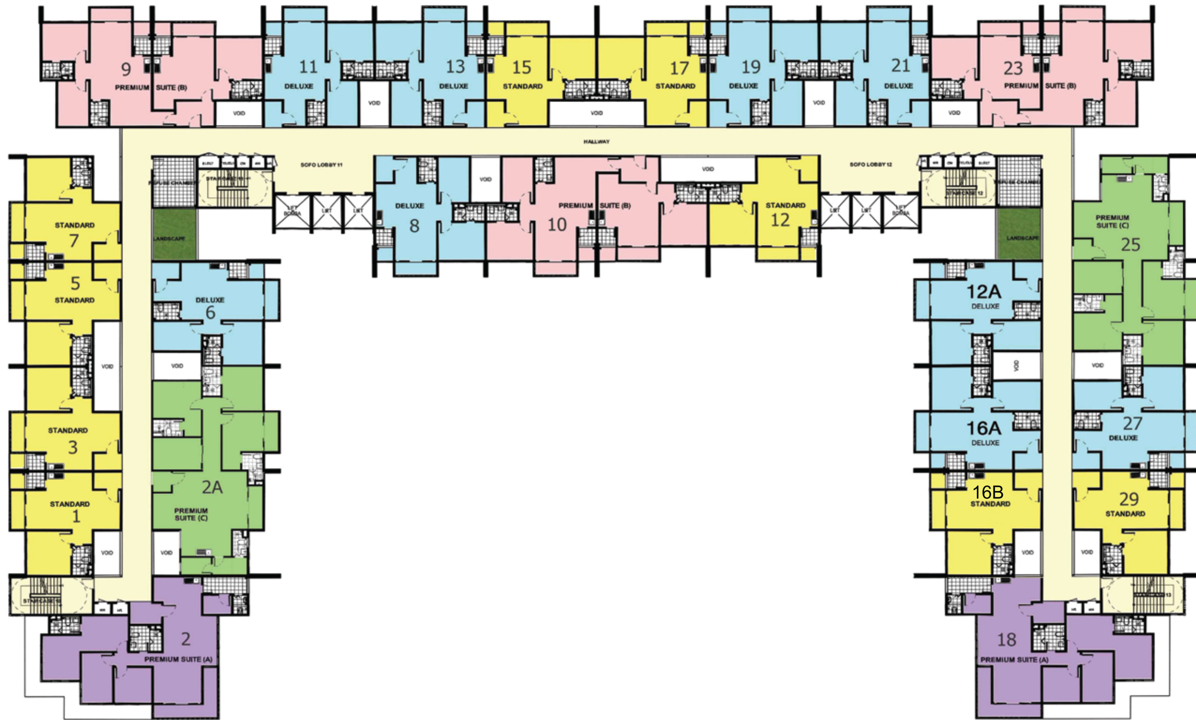
BLOCK A TYPICAL FLOOR PLAN
